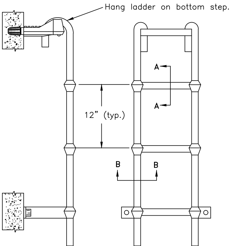
HANGING LADDER
