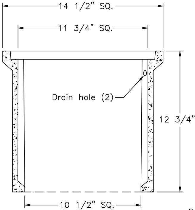
CLEANOUT BOX
