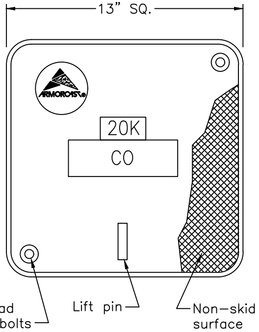
CLEANOUT COVER
