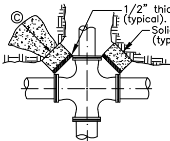
UNBALANCED CROSS
