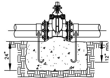
INLINE VALVE - PROFILE
